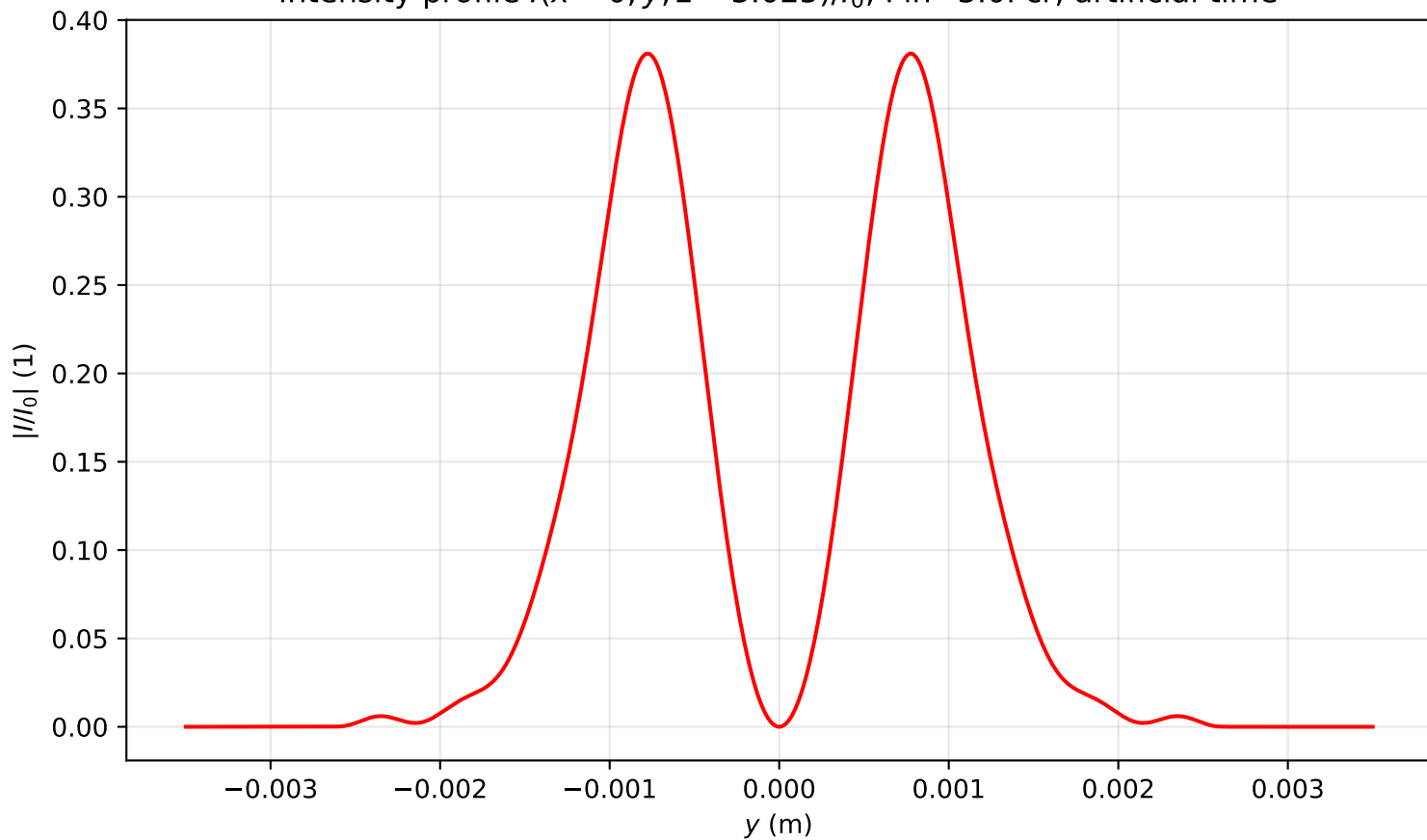
Intensity profile I(x=0, y, z=3.025)/I_0 , \text{Pin}=3.0\text{Pcr} , artificial time
